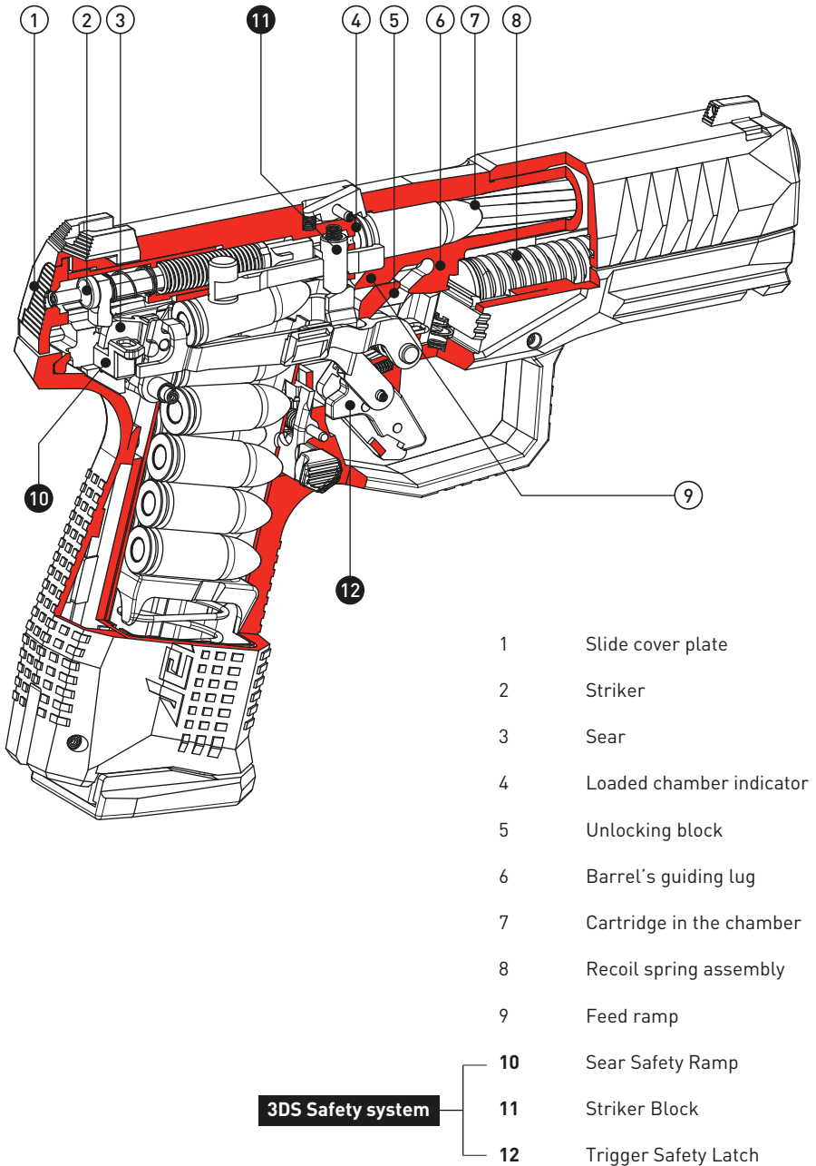
Figure 1 — AREX delta (cutaway view)
